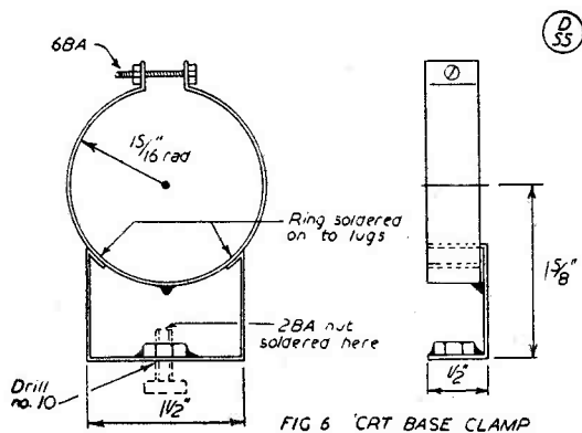
FIG 6 CRT BASE CLAMP
