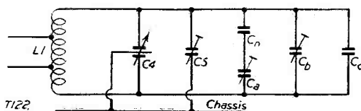
Fig. 2. The circuit of Fig. 1 introduced in the original LFO as shown on p. 395 of the September 1954 issue. C6 in that circuit is replaced by Cc above. C4, C5 are as in the original, Ca is 120 \mu\text{F} , Cb 25 \mu\text{F} , Cc is a 90 \mu\text{F} condenser from a TU5B and Cn is a 270 \mu\text{F} negative temperature coefficient condenser, as discussed in the text.
