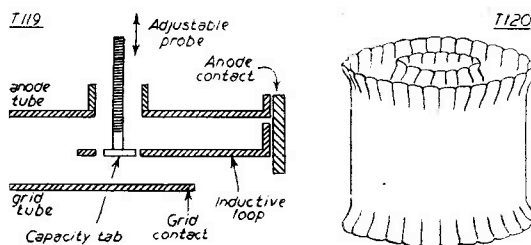
Fig. 7. Showing (left) one method of obtaining a combination of capacity and/or inductive pick-up on the output side. At right is Fig. 8, representing a tuning plunger, or "finger," constructed as described in the text. The lips are sprung to give firm, smooth contact on the walls of the tubes.
