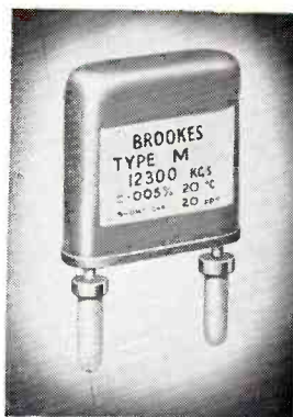
Illustrated above is a Type M Crystal Unit from a range covering 8-20 Mc/s. and on the right is a Type M.I. Crystal Unit from a range covering 8-20 Mc/s.
