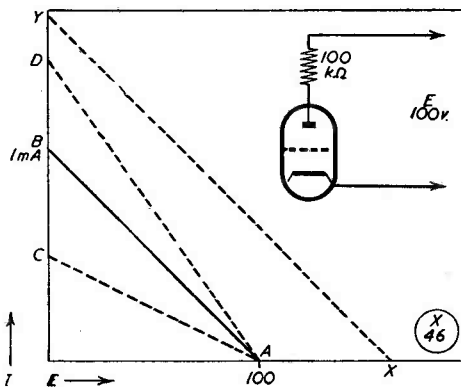
Fig. 3. Typical load-lines. A-B shows a load-line with a 100,000-ohm resistor and 100 volts HT; the lines A-C and A-D are as obtained with different values of resistance but keeping the HT constant. X-Y is a line taken with the 100,000-ohm resistor but increased HT voltage. A-B and X-Y are always parallel, this applying to any load-lines taken with the same resistor but different HT voltages.
