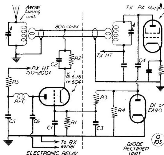
Fig. 2. Electrical layout of the electronic aerial relay suggested by G3GNY. The relay unit, co-ax line, receiver and transmitter must be bonded together. It should be noted that, in his case, the system has only been tried — albeit successfully and over a period — with low power.
