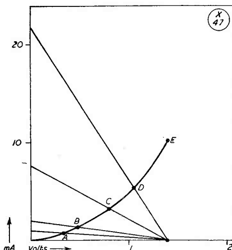
Fig. 4. The curve obtained using the load-line method described by G2HR. Points A, B, C and D show current through the resistor and diode together, and point E the current through the diode only. In this case, the battery voltage was 1.4.
